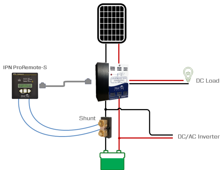
IPN ProRemote-S example of installation
