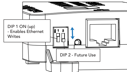
Figure 2-3. DIP Switch Functions
