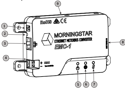
Figure 1-1 EMC-1 Features
