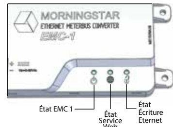
Figure 3-1. Voyants DEL
